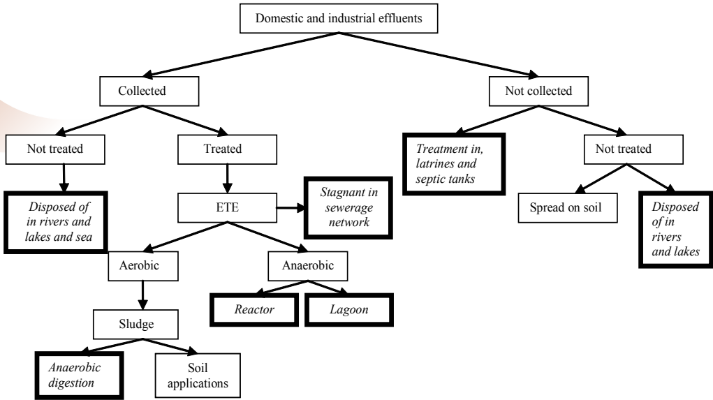
Figure 34 - Sources of sewage and effluents, treatment systems and potential CH 4 emissions
